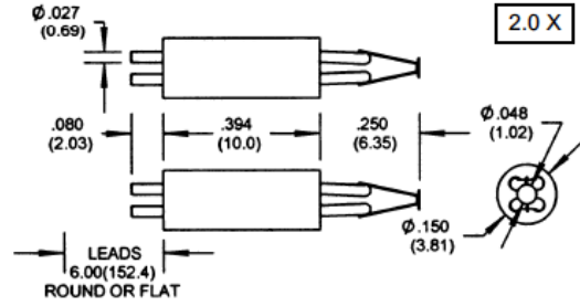
ES-044 Tantalum Disc Cathode mounted on a high current CB-105 ceramic base
