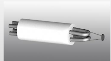
Tantalum Disc Cathode ES-044 mounted on a CB-105 base.
