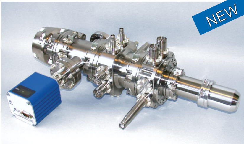
EMG-4103 Electron Gun, 4½ CF or 6 CF mounting flange, (optional ion gauge and custom flange shown)
