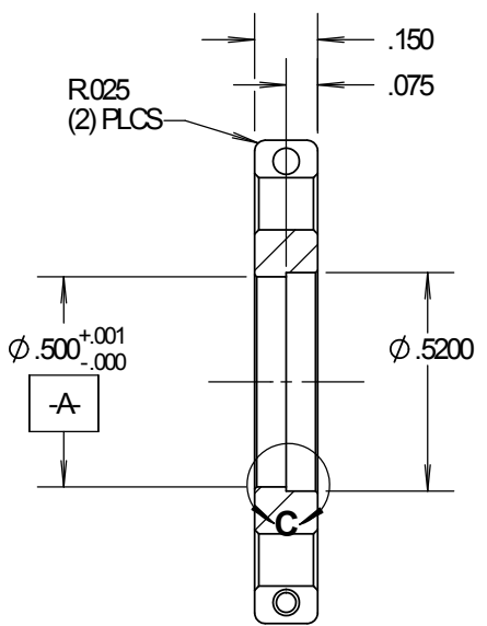
SECTION B-B (VIEW ROTATED 45° CCW)
