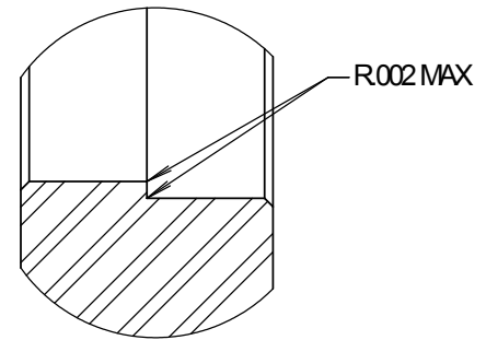
DETAIL C SCALE 8:1
