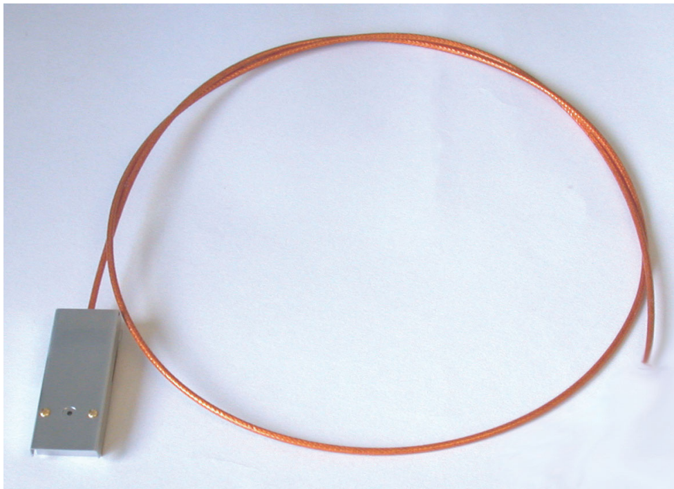
FC-70C Faraday Cup and UHV cable with one end unterminated (0.5X)
