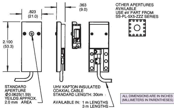
FC-70C Faraday Cup and UHV cable with one end unterminated (0.5X)
